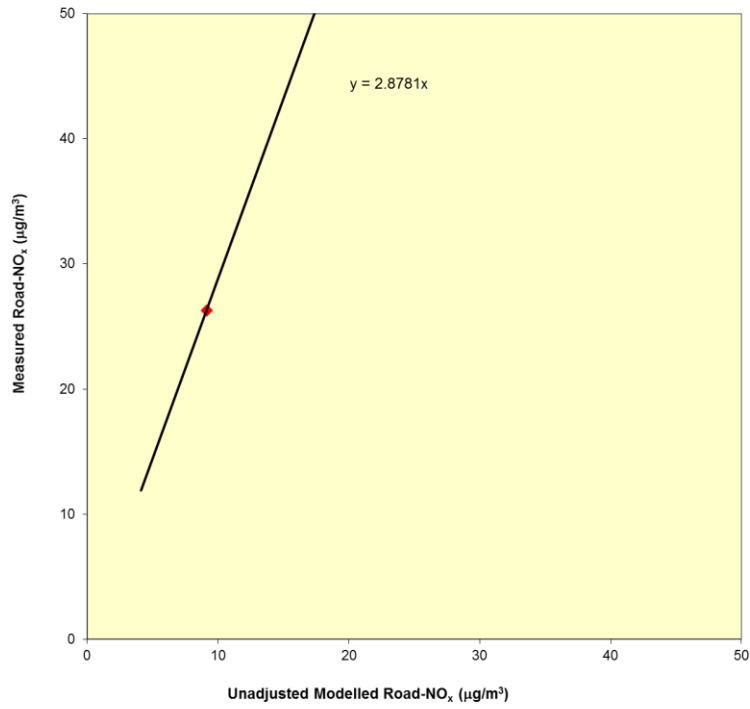
Figure C.1.4.1: Comparison of Measured Road-NO x with Unadjusted Modelled Road-NO x Concentrations
